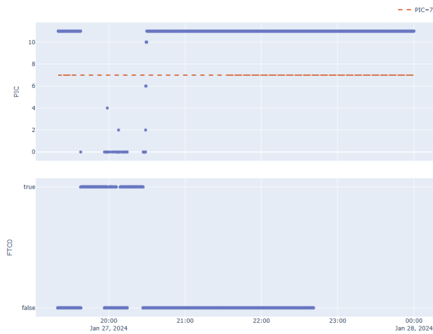
FIGURE 12 Flight CSC3816 on 2024-01-27 - Timeline of the PIC and FTC0 data
