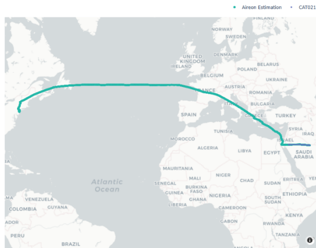
FIGURE 13 Flight UAL163 on 2024-11-16 - Independent estimation of position (green) vs reported ADS-B data (purple)
