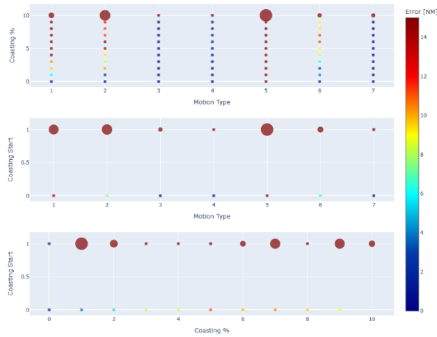
FIGURE 3 Performance analysis per trajectory type: 95 th percentile error
