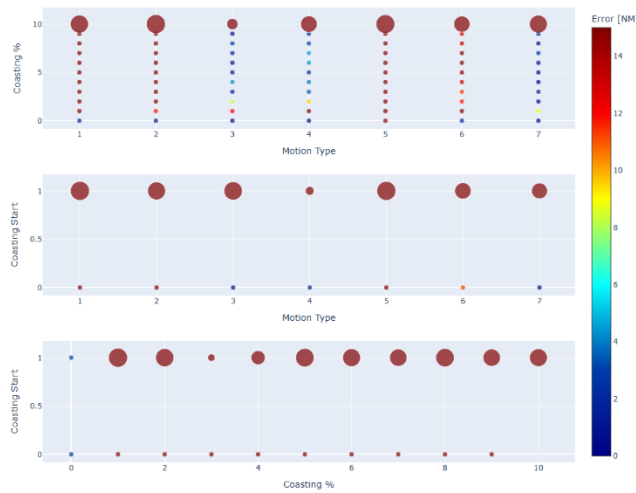
FIGURE 4 Performance analysis per trajectory type: 98 th percentile error
